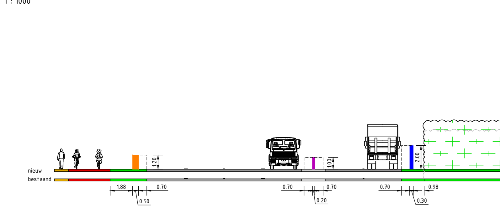
PRINCIPEPROFIEL 1-1 VARIANT 2
