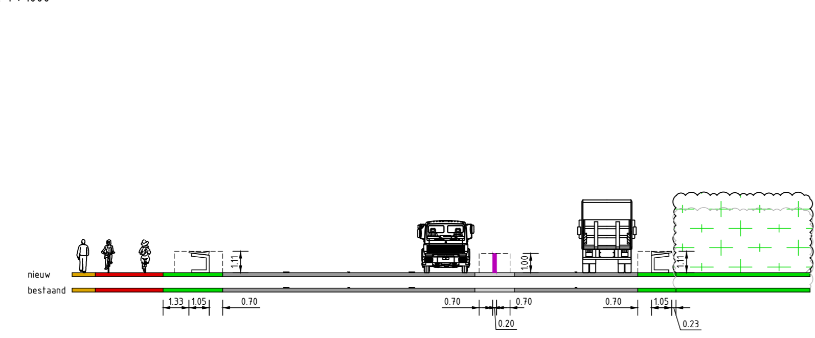
PRINCIPEPROFIEL 1-1 VARIANT 1
