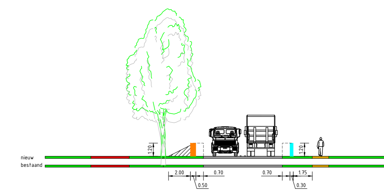
PRINCIPEPROFIEL 4-4 VARIANT 2
