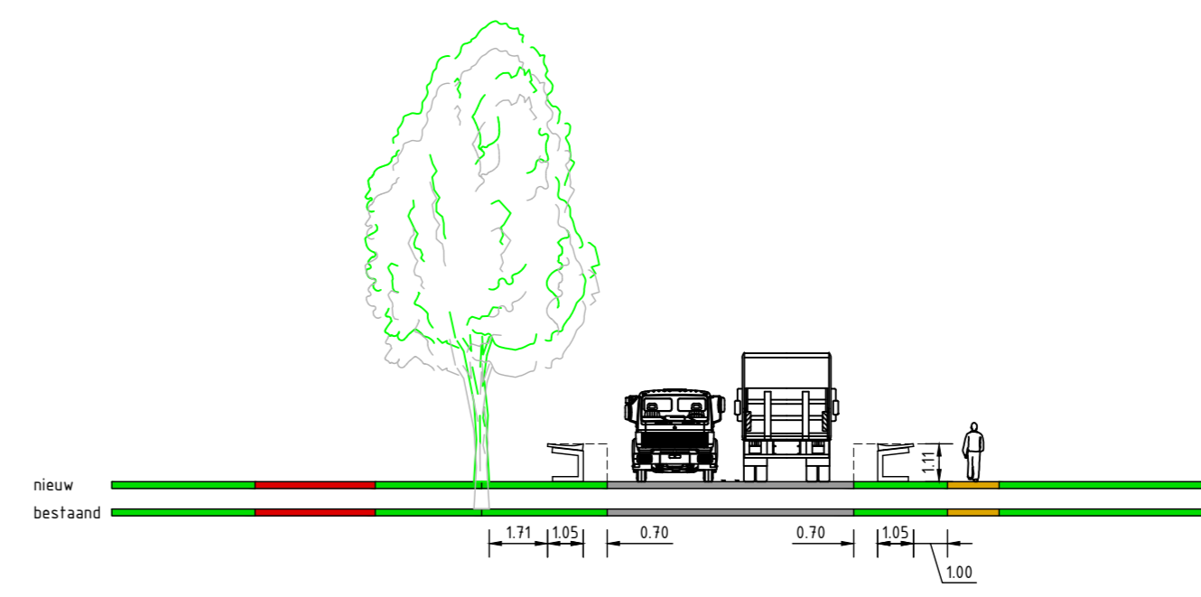
PRINCIPEPROFIEL 4-4 VARIANT 1
