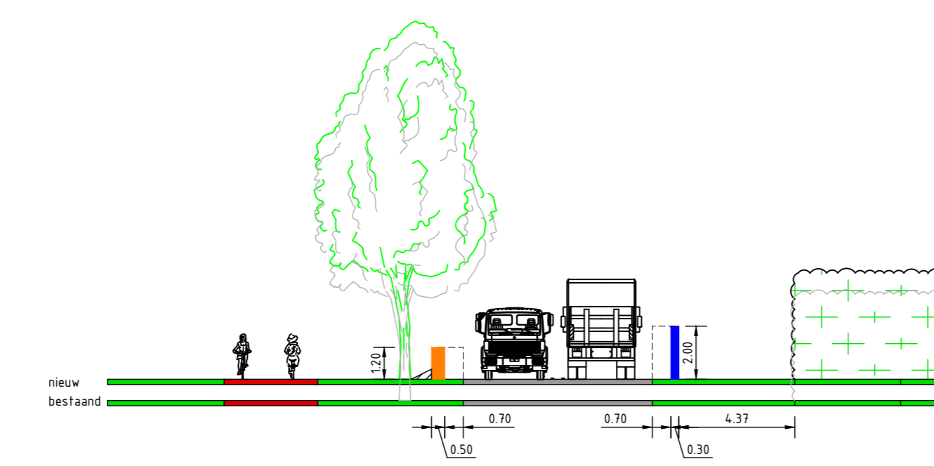
PRINCIPEPROFIEL 2-2 VARIANT 2
