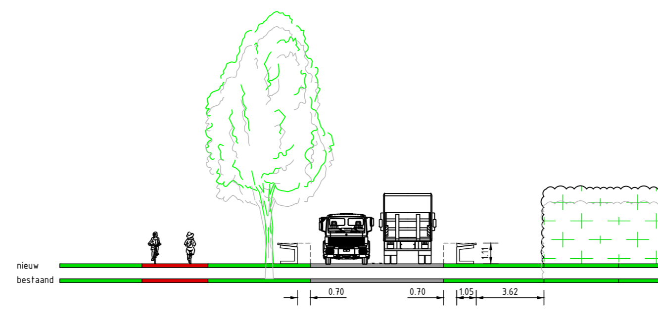
PRINCIPEPROFIEL 2-2 VARIANT 1
