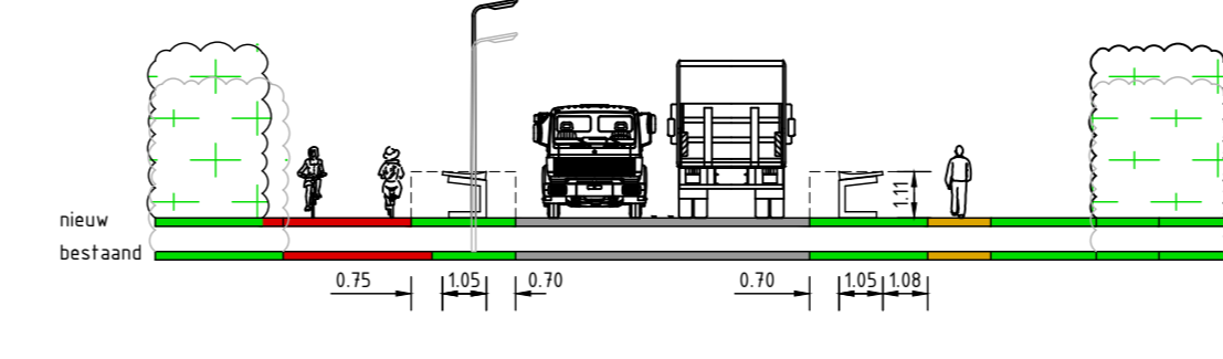
PRINCIPEPROFIEL 3-3 VARIANT 1
