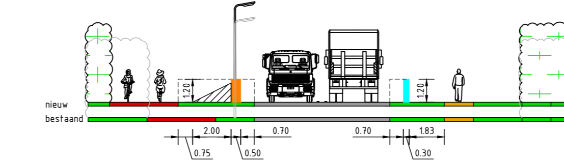
PRINCIPEPROFIEL 3-3 VARIANT 2
